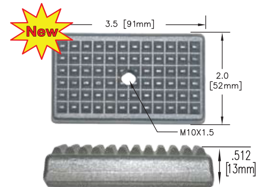
Beretta Jaw Pads TD15X52-92F-I
